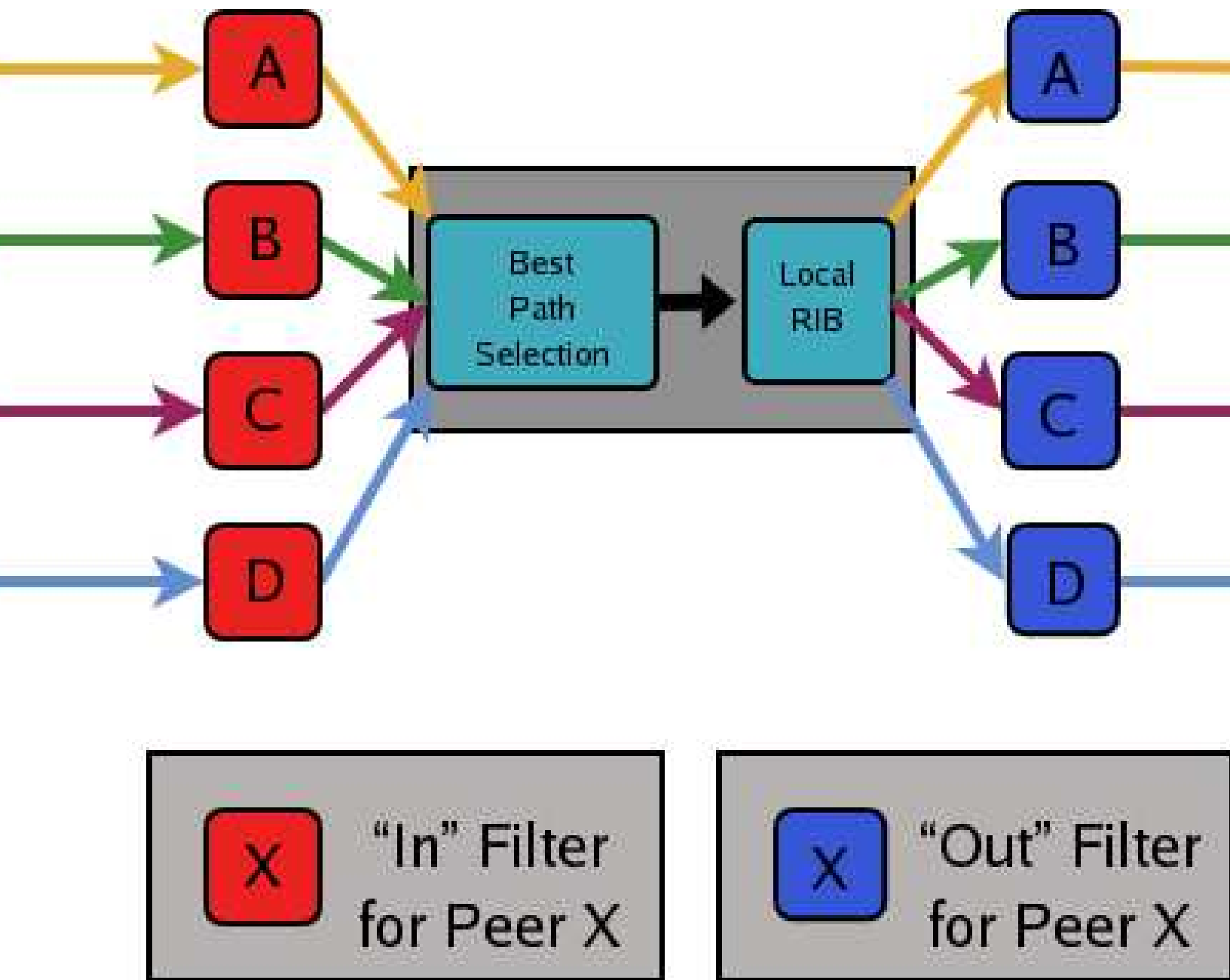
Figure 10.1: Announcement processing inside a "normal" BGP speaker
